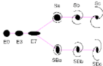
Hubble "Tuning Fork" Diagram
